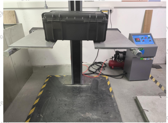
Test set-up
