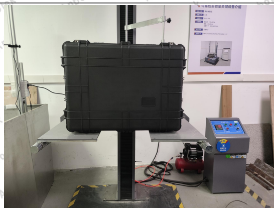
Test set-up
